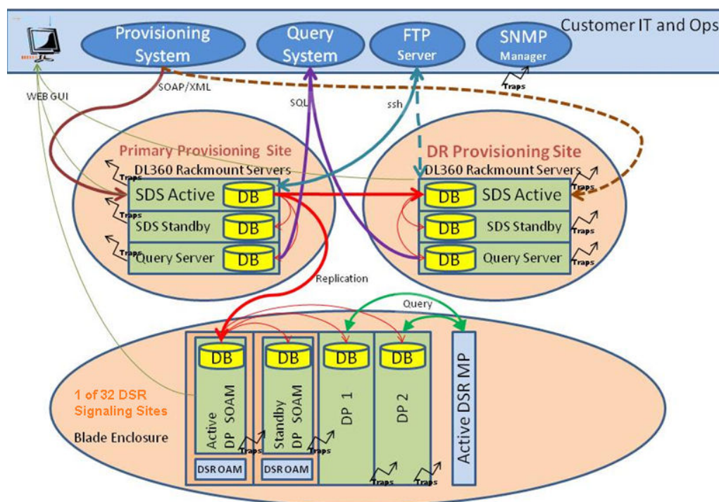
Figure 2-1 SDS System Diagram
